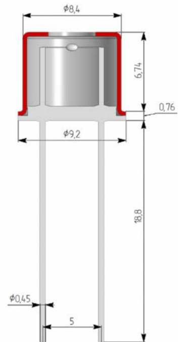
All measurements in mm.
